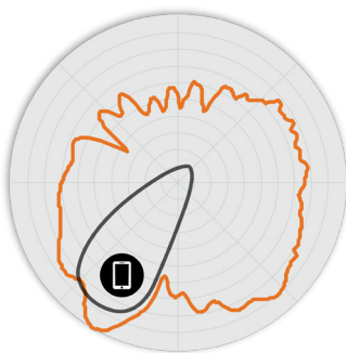
Figure 6. R770 5GHz Elevation Antenna Patterns
