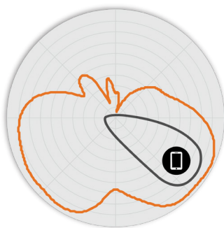
Figure 5. R770 2.4GHz Elevation Antenna Patterns
