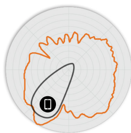
Figure 6. R670 5GHz Elevation Antenna Patterns
