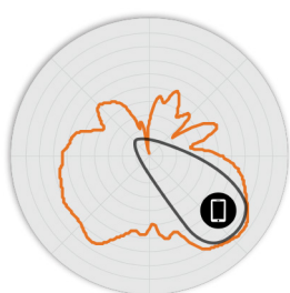
Figure 7. R670 6GHz Elevation Antenna Patterns
