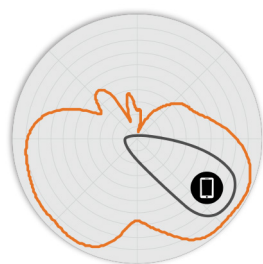
Figure 5. R670 2.4GHz Elevation Antenna Patterns
